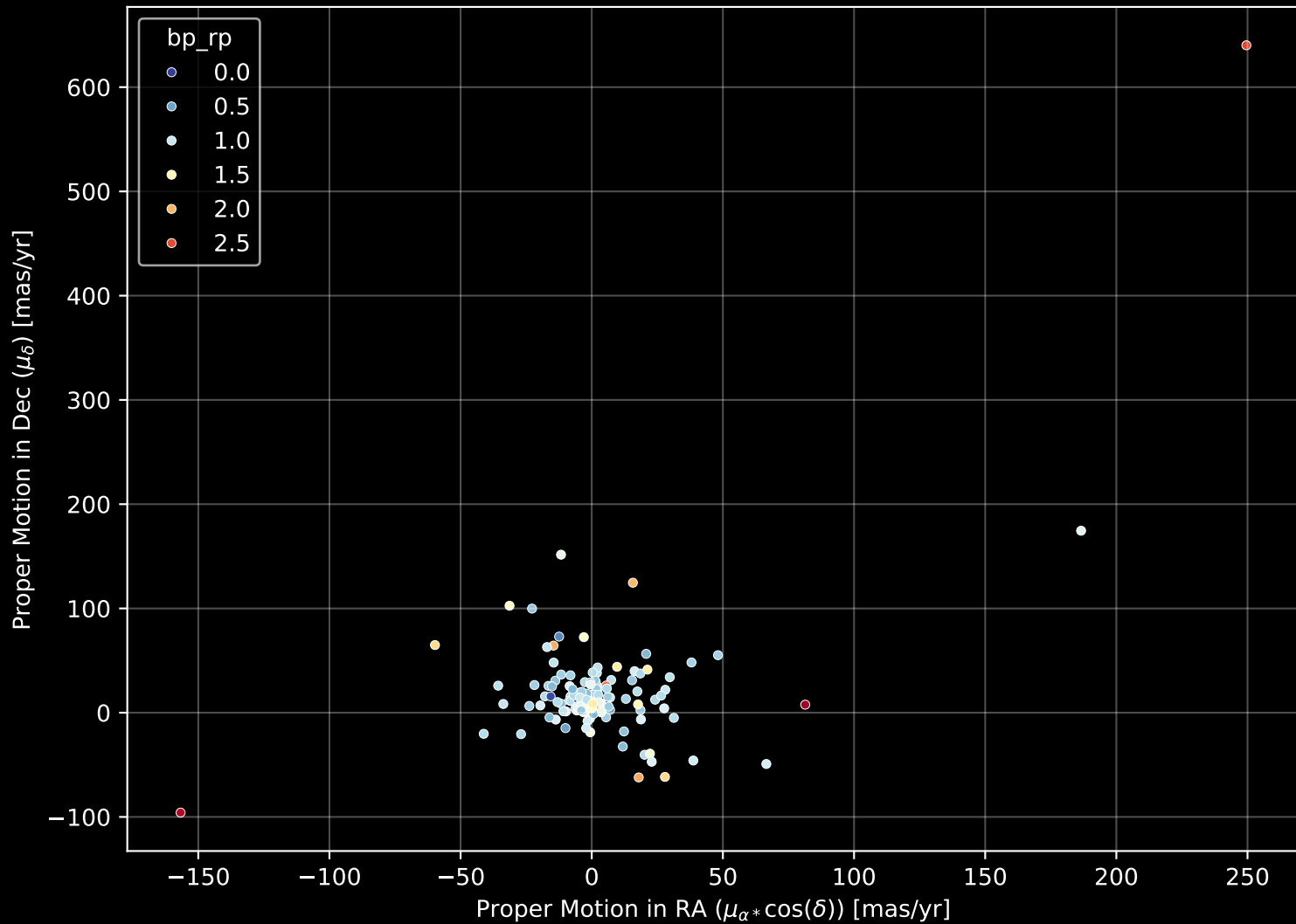
APOGEE DR17 Field: [280-26-O_TESS] Proper Motion Diagram (n= 156)
