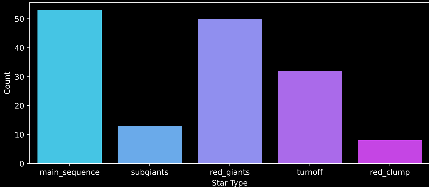
APOGEE DR17 Field: [280-26-O_TESS] Count plot of Star Type
