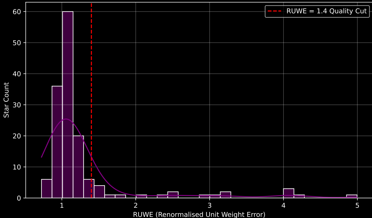
GAPOGEE DR17 Field [280-26-O_TESS] RUWE Distribution (n= 147)
