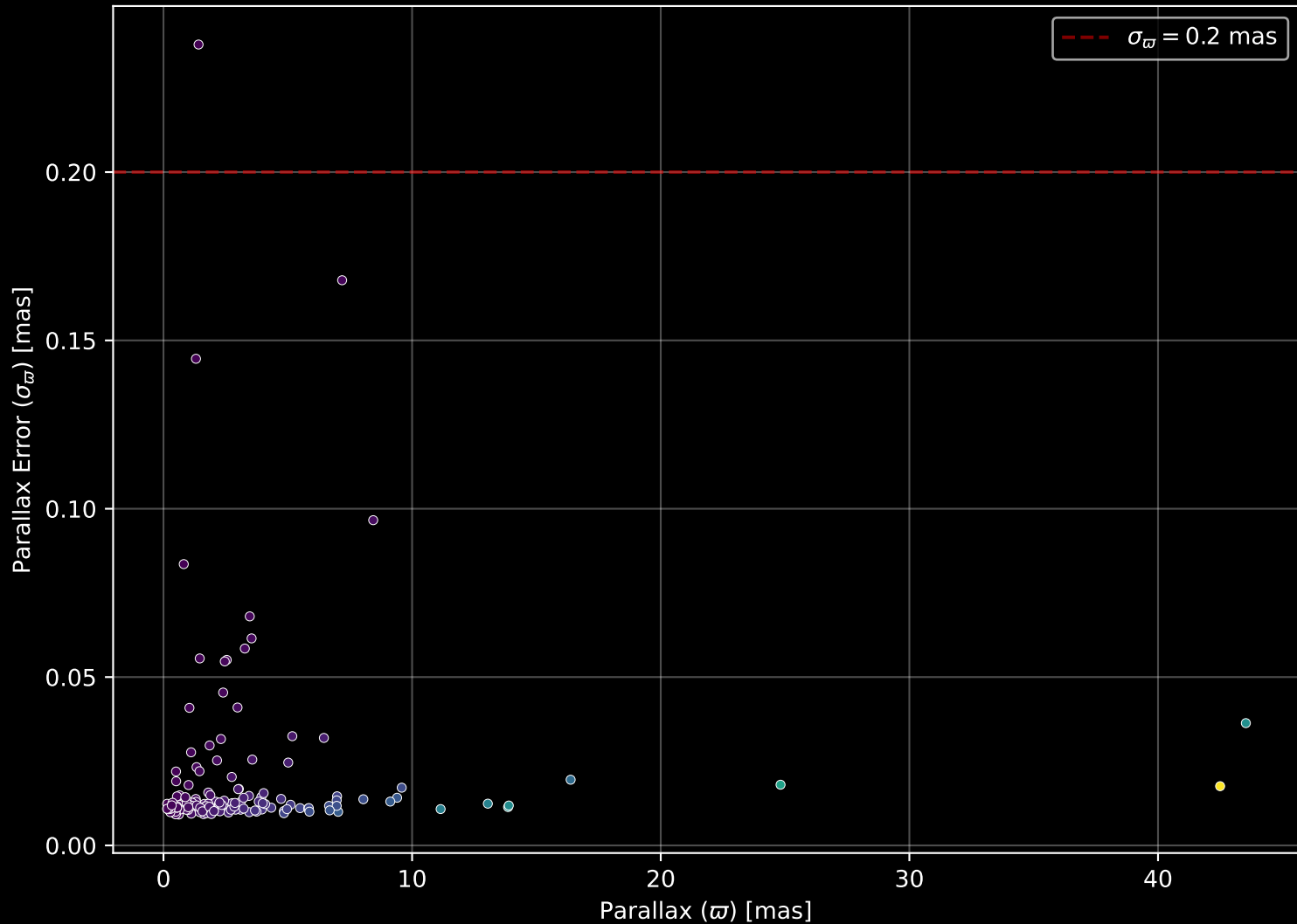
APOGEE DR17 Field: [280-26-O_TESS] Parallax Quality (n= 156)
